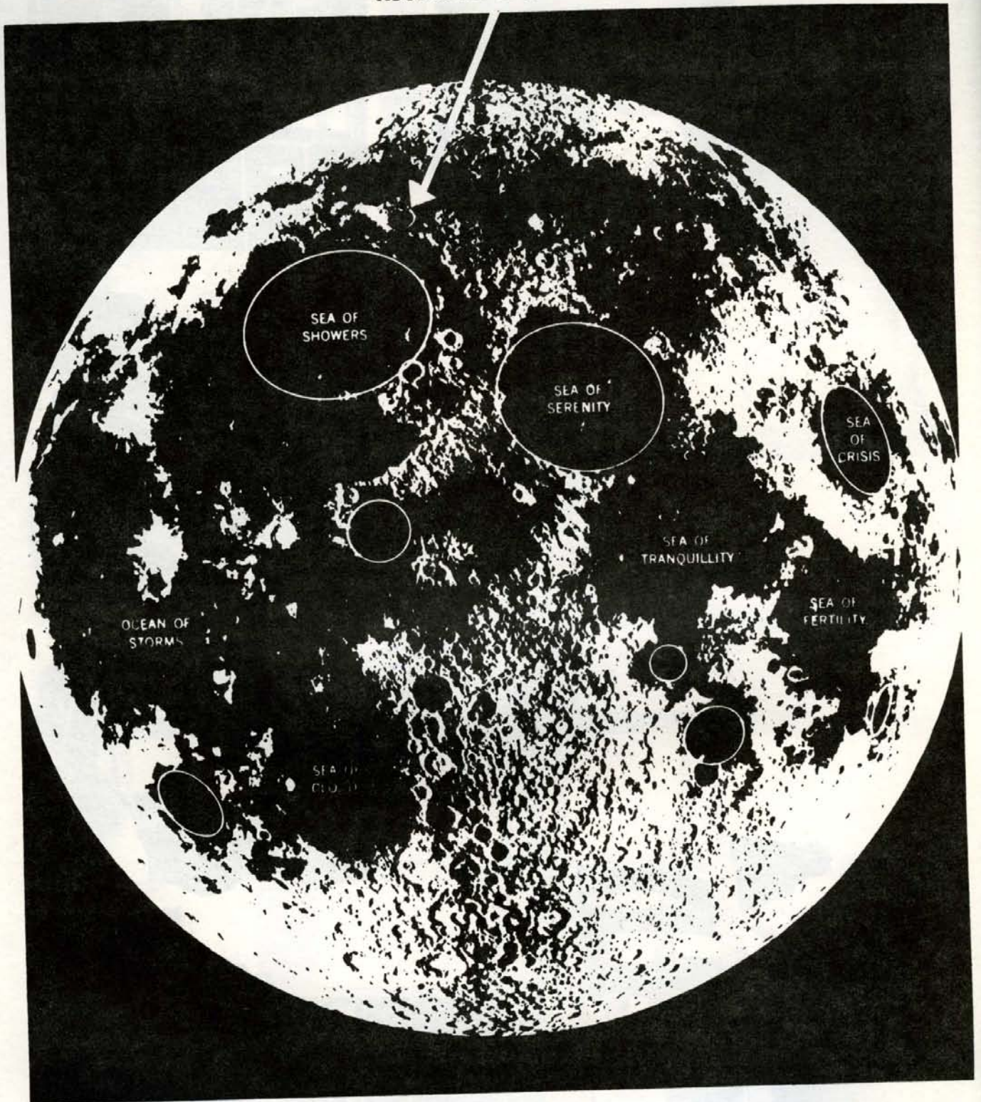
Moonbase Alpha in crator Plato
